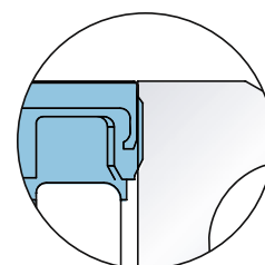
Bolt-Hole without Chamfer (optional: /TR)
