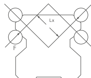
X-Type Arrangement
