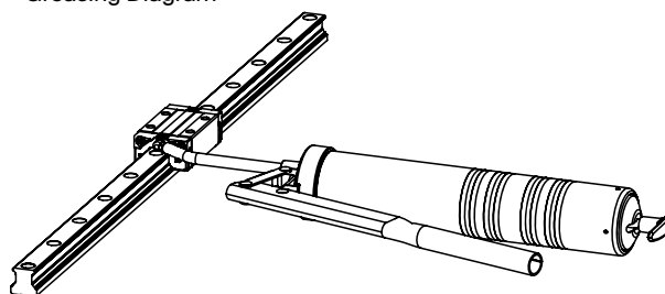
Greasing Diagram
