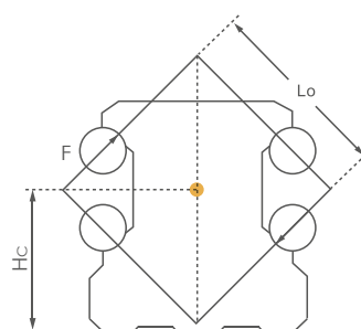
O-Type Arrangement
